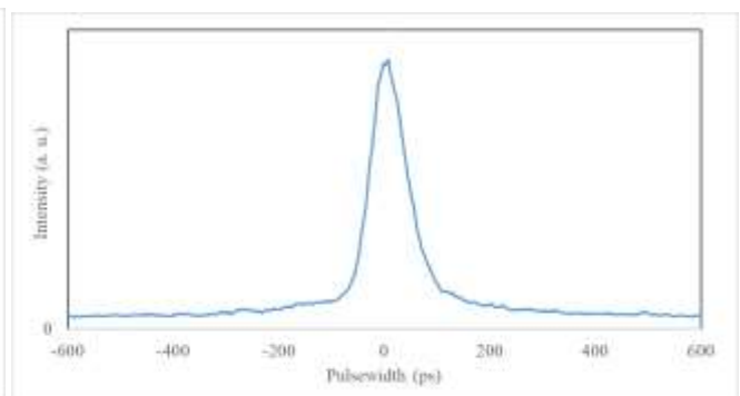
OEPLS-PS-100 spectrum and pulse shape at 1060 nm.
