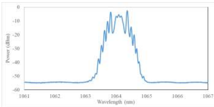
OEPLS-PS-100 spectrum and pulse shape at 1060 nm.
