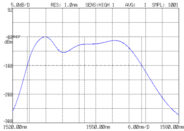
OEBS-100-1550 (C band)
