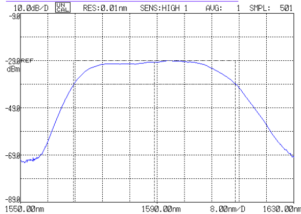
OEBS-100-1590 (L band)
